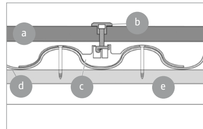
Horizontal section
