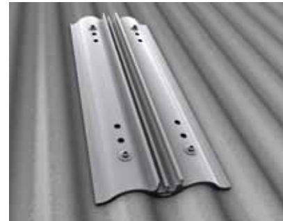
Adapter for module orientation landscape with Quickstone channel
