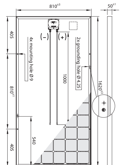
frame section
